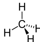
Methane CH 4
